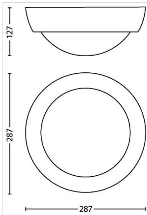
Figure 2: Dimensions diagram for Philips Celestial Ceiling Lamp. Technical drawing illustrating the dimensions of the Philips Celestial ceiling lamp. The lamp has a diameter of 287mm and a height of 127mm.
