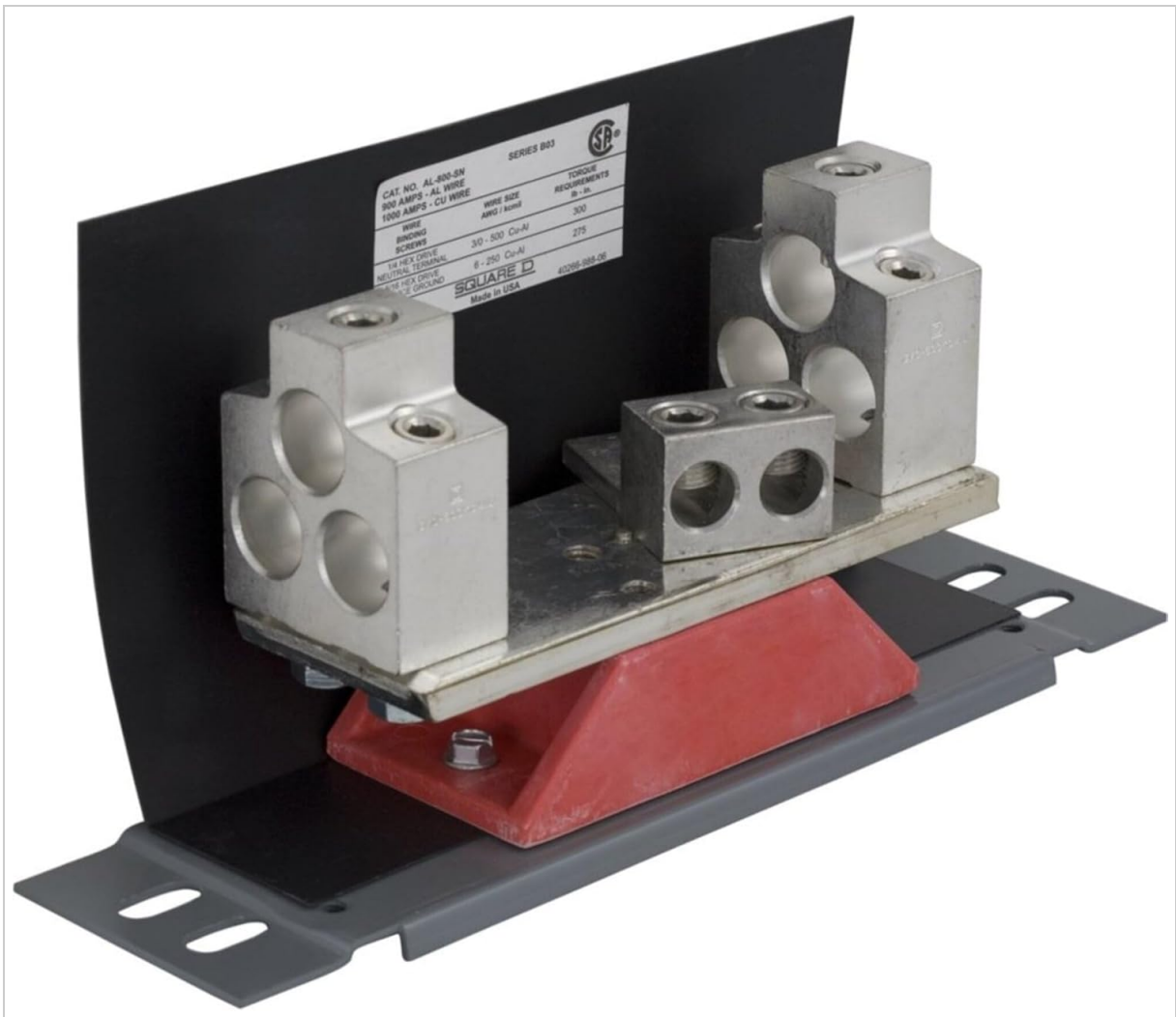
Figure 1: Schneider Electric AL800SN 1000-Amp Neutral Assembly. This image displays the complete neutral assembly, featuring multiple wire connection points, a robust base, and clear labeling for specifications and torque requirements.
