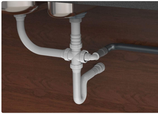
Image: A close-up view illustrating the flexible design of the pipe, allowing it to be shaped into a P-trap.
