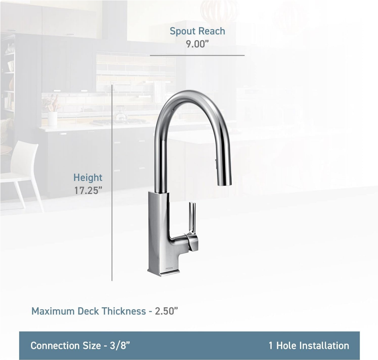
Image: Faucet dimensions for installation planning.
