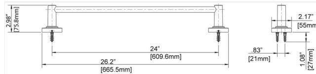
Illustration of preparing the mounting posts and marking the wall.
