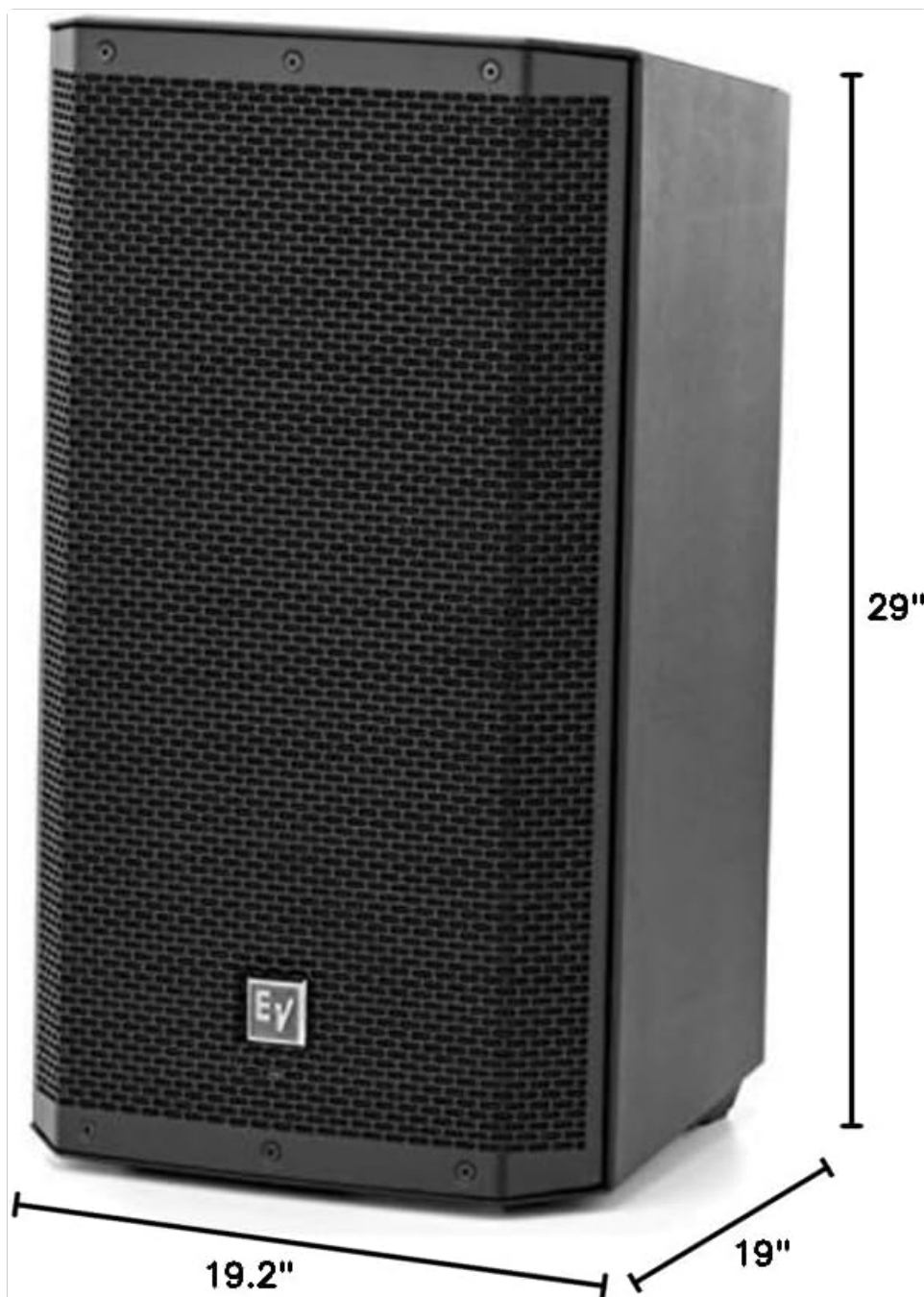
Figure 7.1: Dimensional overview of the ZLX-15P loudspeaker.
