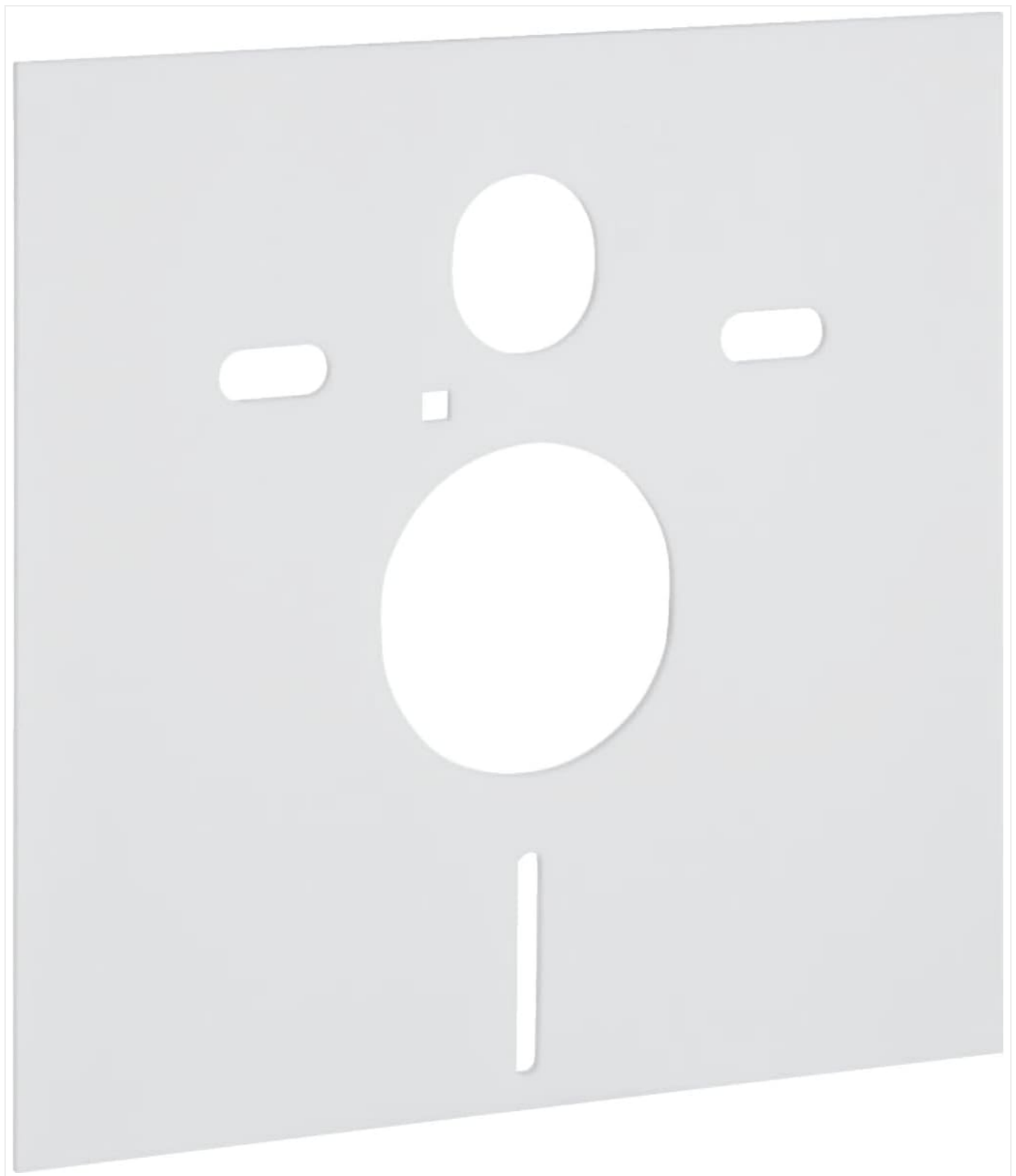
Figure 1: Geberit G156050001 Acoustic Insulation Set. This image displays the white insulation pad with cutouts for mounting bolts and plumbing connections, designed to fit between a wall-mounted ceramic fixture and the wall.
