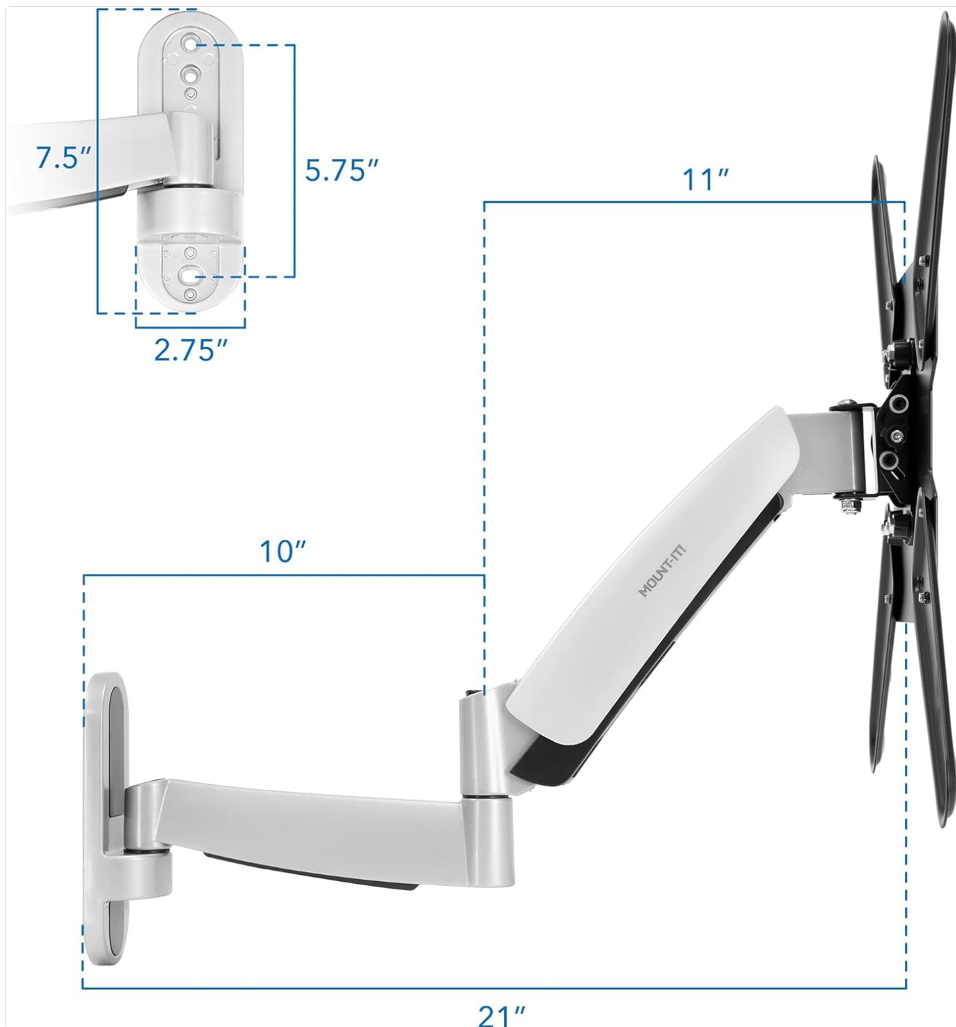
Image: Detailed dimensional drawing of the Mount-It! TV mount, showing arm lengths, wall plate size, and overall extension.
