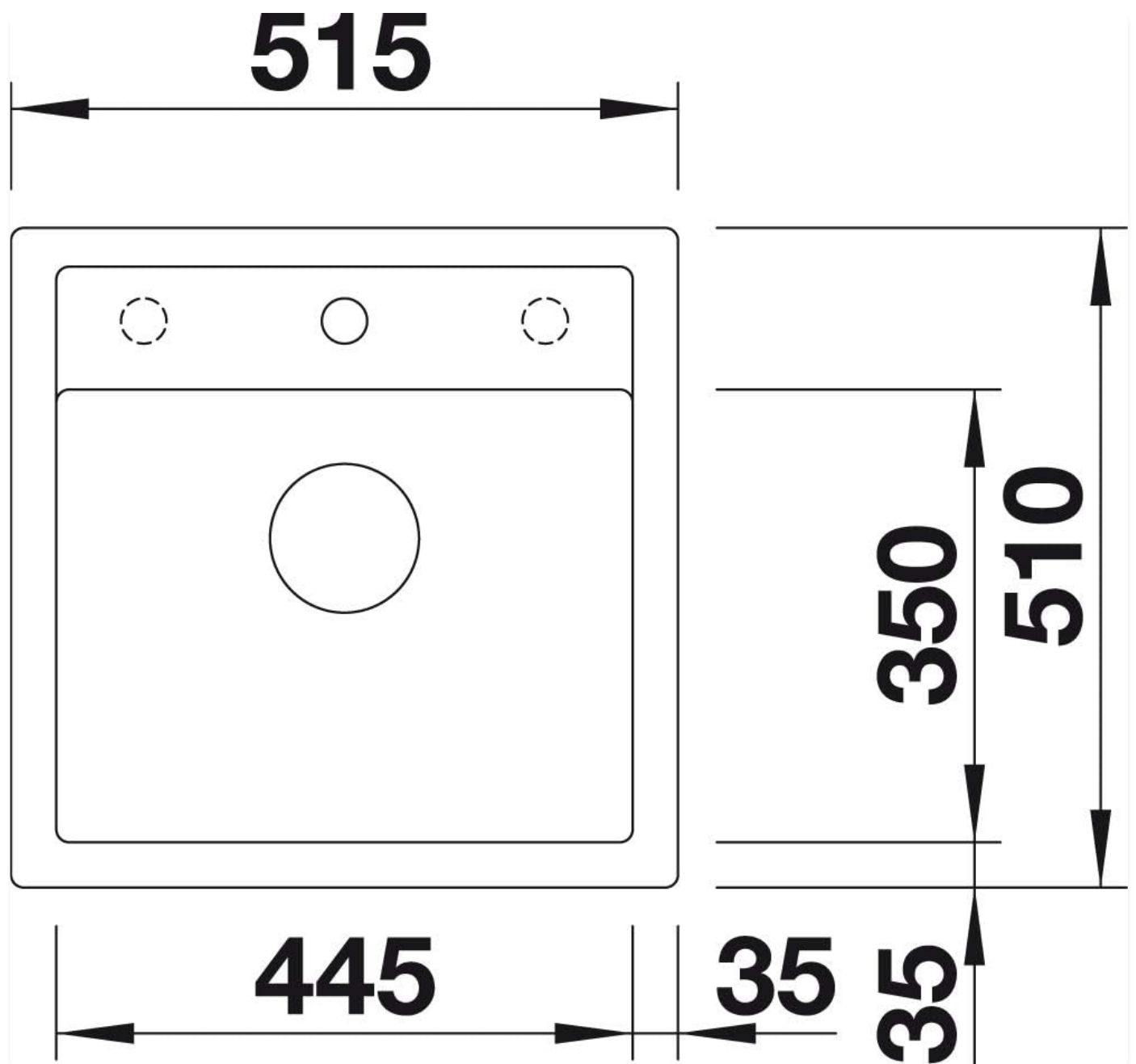
Figure 2.1: Top view dimensions of the sink (515mm x 510mm overall, 445mm x 350mm bowl).
