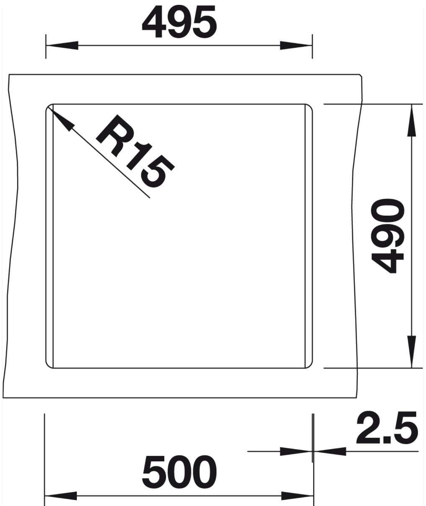
Figure 2.2: Countertop cutout dimensions (495mm x 490mm with R15 corners).
