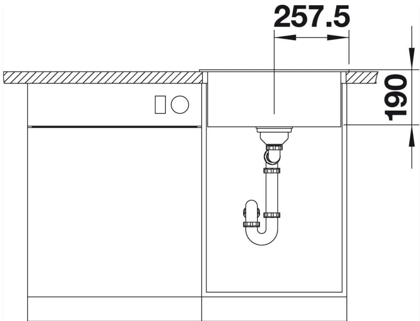
Figure 2.3: Side view installation diagram, showing sink depth (190mm from top of counter to bottom of sink) and plumbing connections.
