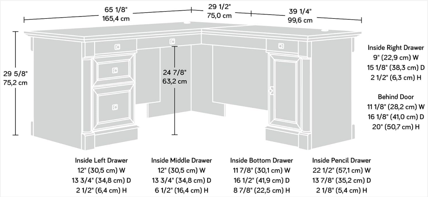
Image: Detailed dimensions diagram of the L-shaped desk, showing measurements for overall size and internal drawer/storage areas.
