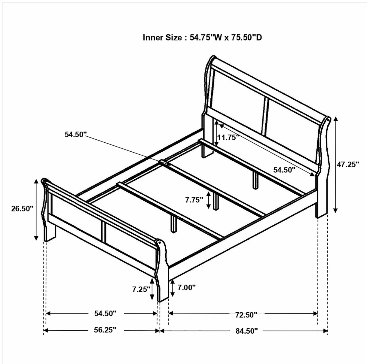
Figure 1: Assembly diagram with key dimensions (84.5"L x 56.25"W x 47.25"H).
