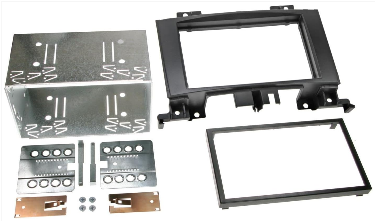
Figure 1: Components of the ACV Electronic 2 DIN Car Radio Fascia Kit. This image displays all components included in the kit, featuring the main black plastic fascia frame, a metal mounting cage, a black plastic trim frame, various metal brackets, and small screws. These parts are essential for securely installing a double DIN car radio into compatible vehicle dashboards.
