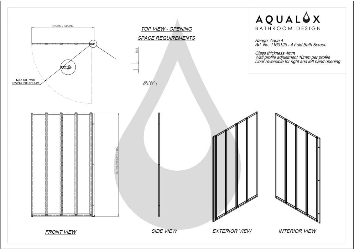
Image: Technical drawing showing front, side, exterior, and interior views of the bath screen, along with top view opening space requirements and dimensions (835mm-845mm width, 1400mm height).
