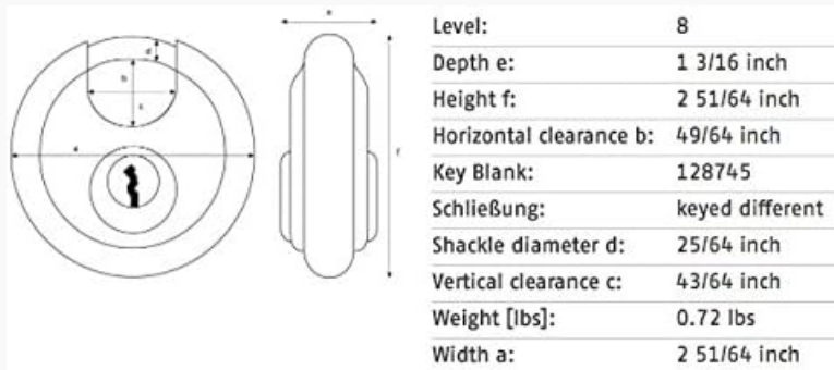
Technical diagram illustrating the precise dimensions of the ABUS 26/70 Diskus Padlock.
