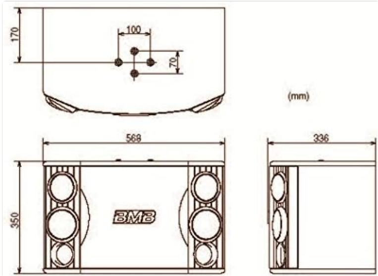
Image: Dimensional drawing of the BMB CSD-880 speaker.
