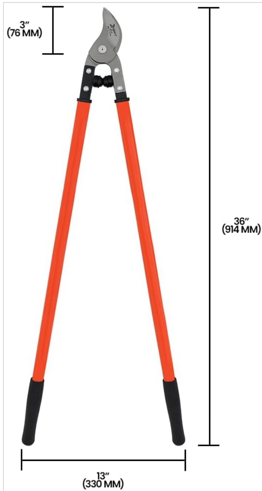
Figure 3: Dimensional overview of the Zenport MV190 lopper, showing its 36-inch length and other key measurements.
