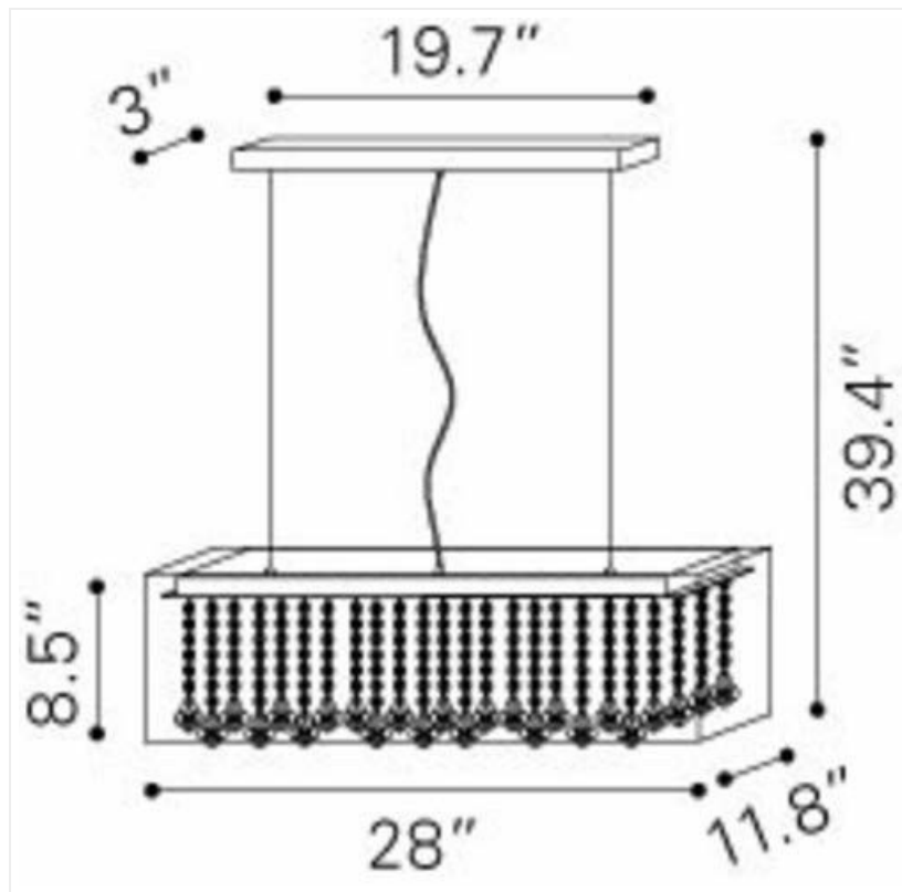
Image 4.1: Dimensional diagram of the Zuo Modern Blast Ceiling Lamp, showing measurements in inches.
