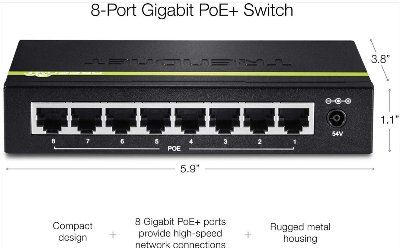
Figure 3: Product Dimensions (5.9"L x 3.8"W x 1.1"H)
