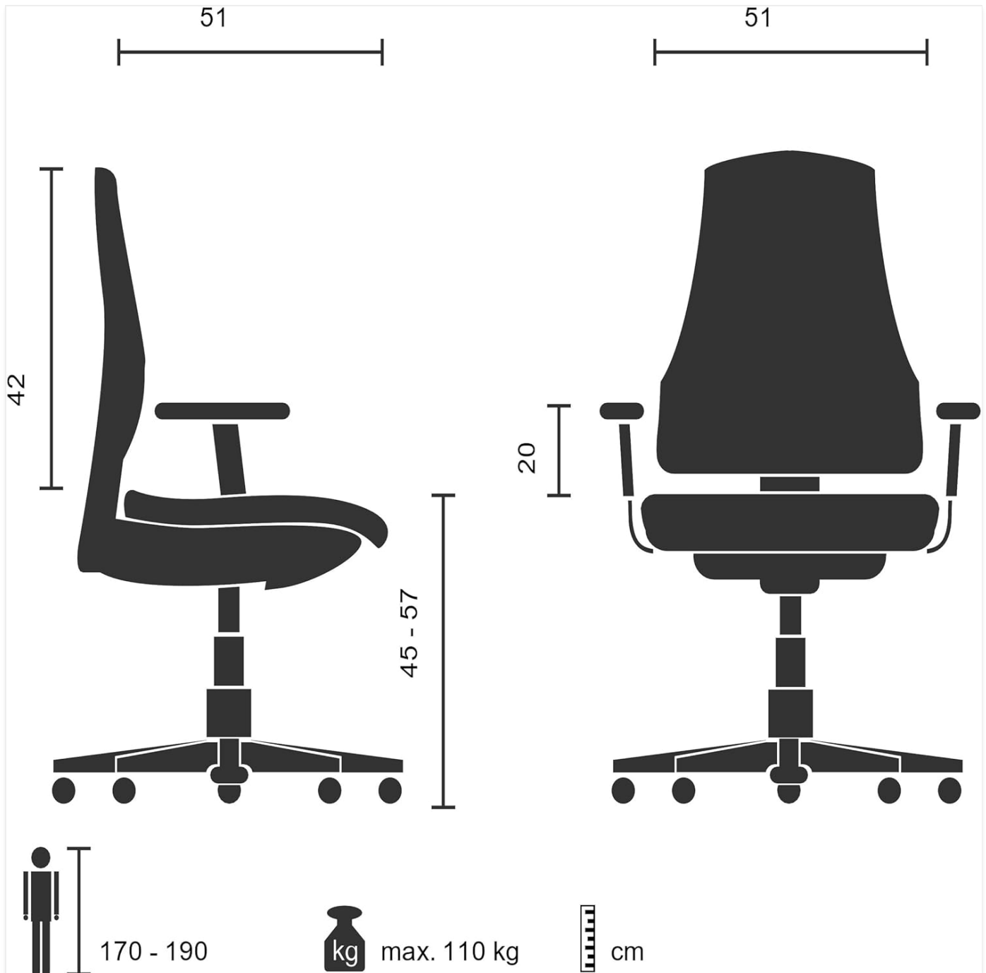
Figure 2: Dimensional overview of the chair, useful for understanding assembly orientation.
