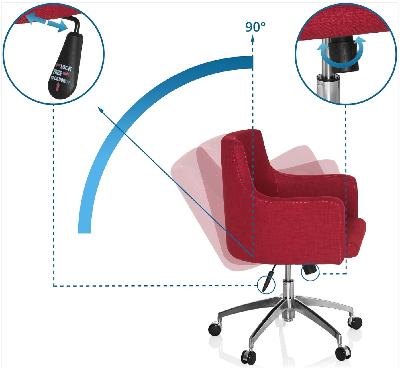
Figure 3: Illustration of the reclining mechanism and its operation.
