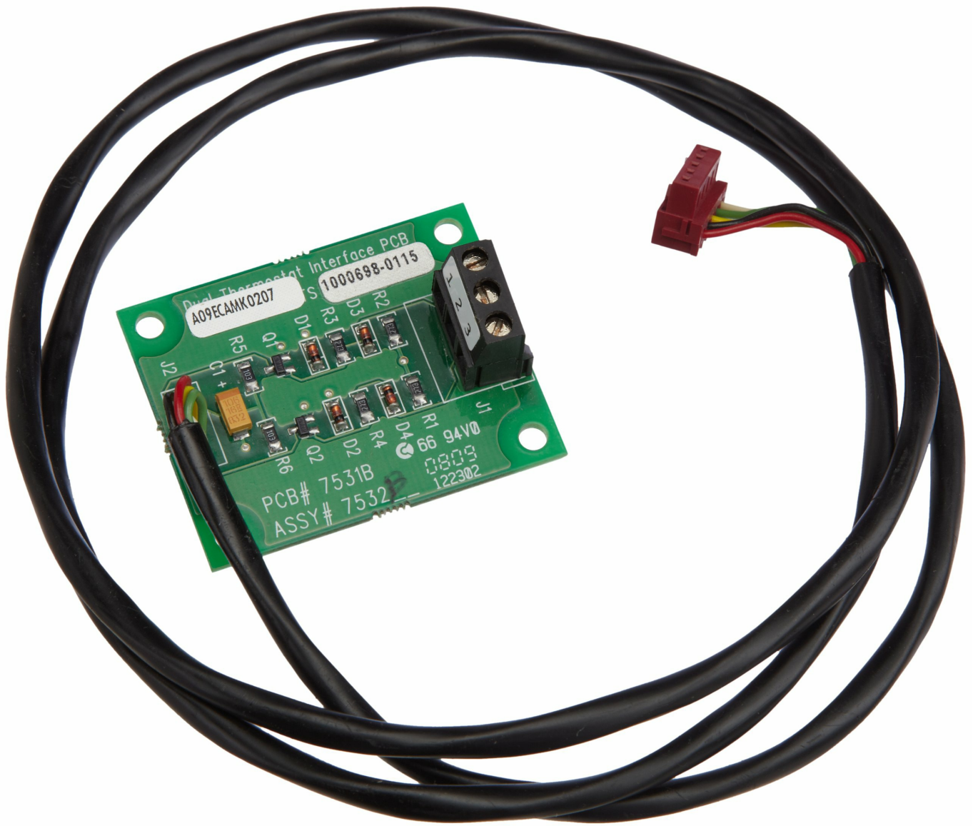
Figure 1: The Zodiac 7727 Dual Thermostat Switch Replacement Kit. This image displays the main component of the kit, which is a small green circuit board (PCB# 7531B, ASSY# 7532) with various electronic components, including resistors and capacitors. Two black insulated wires extend from the board, one terminating in a red four-pin connector, and the other connected to a screw terminal block on the board. The board is labeled "Dual Thermostat Interface PCB" and includes part number S1000698-0115.
