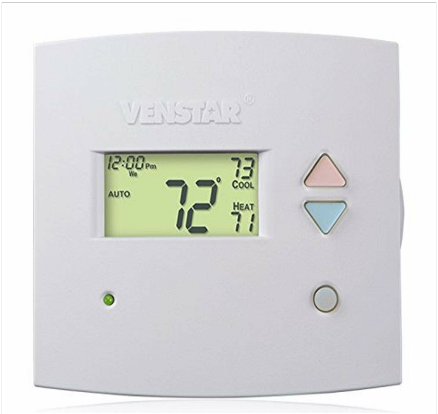
Front view of the Venstar T2800 thermostat, displaying the current time, day, ambient temperature, and set temperatures for cooling and heating. It features up and down arrow buttons for temperature adjustment and a mode button.
