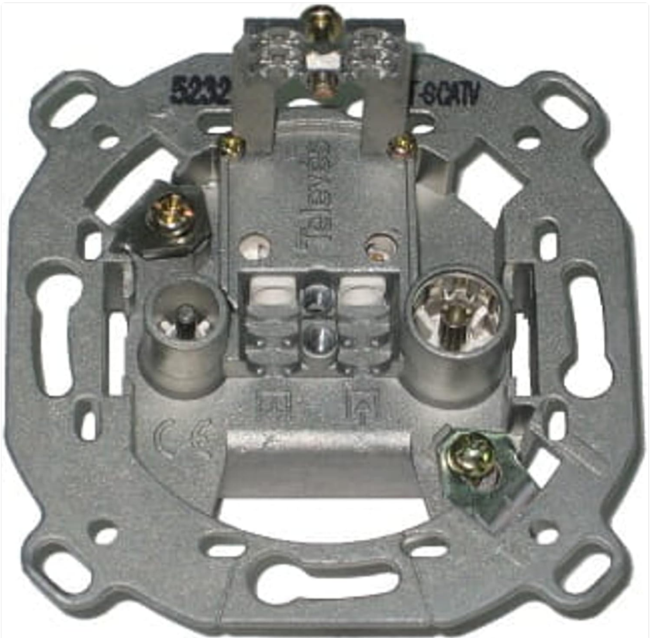
Figure 2: Detailed view of the metal mounting frame, highlighting the internal wiring terminals and model identification.
