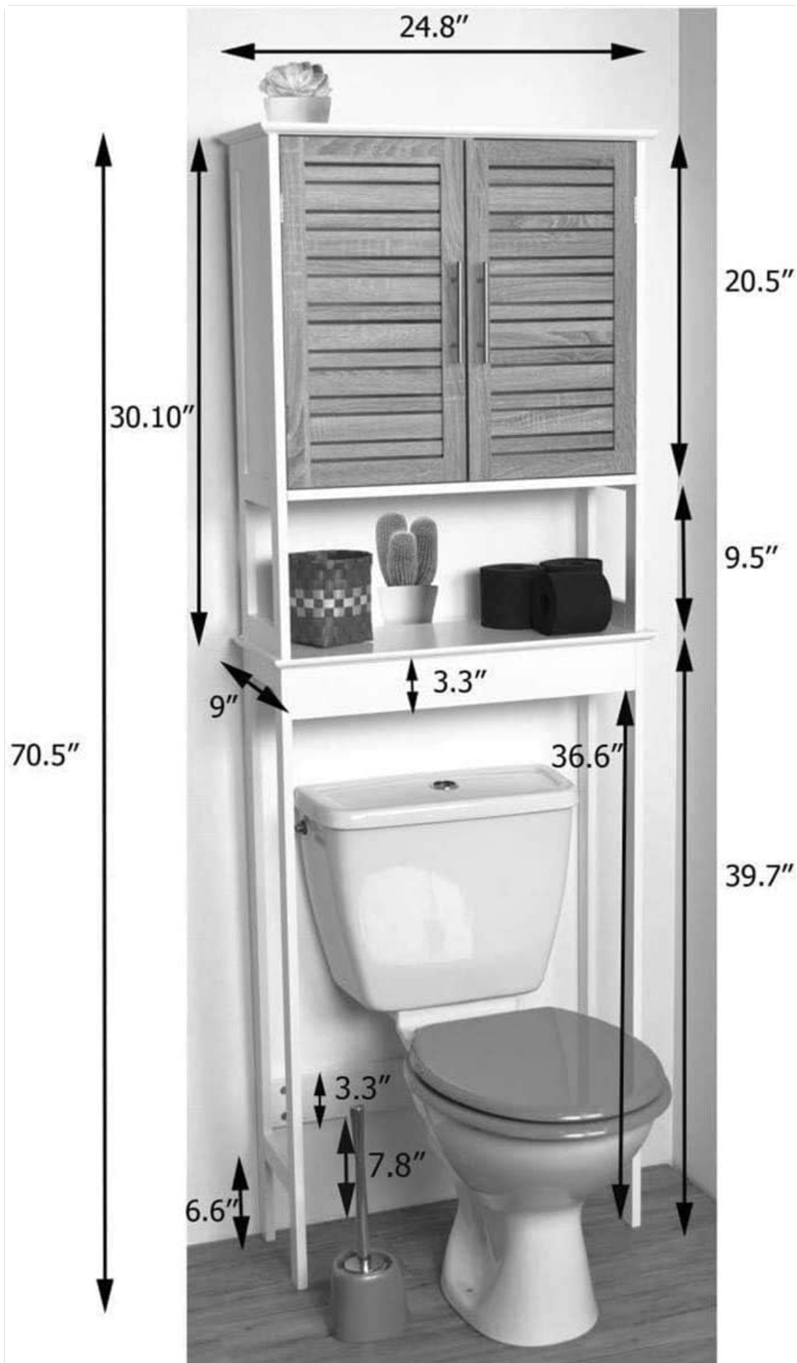
Image 2: Dimensional Diagram. This diagram illustrates the key measurements of the cabinet, including overall height, width, depth, and internal shelf spacing, which are crucial for assembly and placement.
