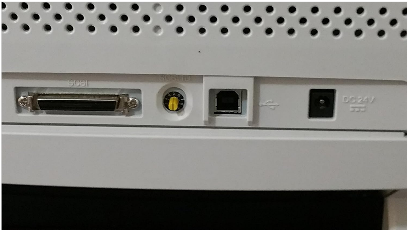
Figure 7: Close-up view of the rear connection ports, including SCSi, SCSi ID selector, USB, and DC 24V power input.
