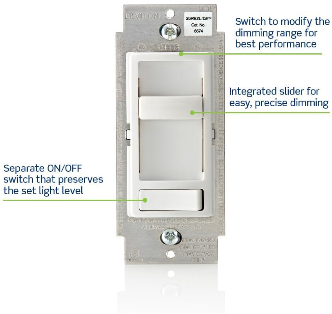
Figure 3.1: Key features of the SureSlide Dimmer, including the integrated slider, separate ON/OFF switch, and mode selector.
