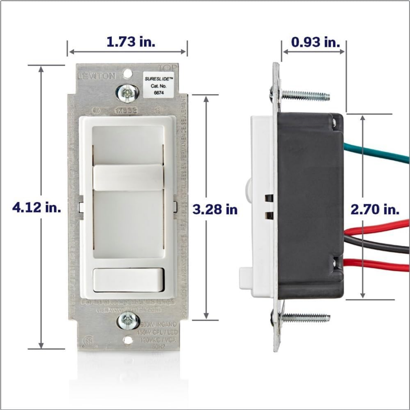
Figure 8.1: Product dimensions for the Leviton SureSlide Dimmer Switch.
