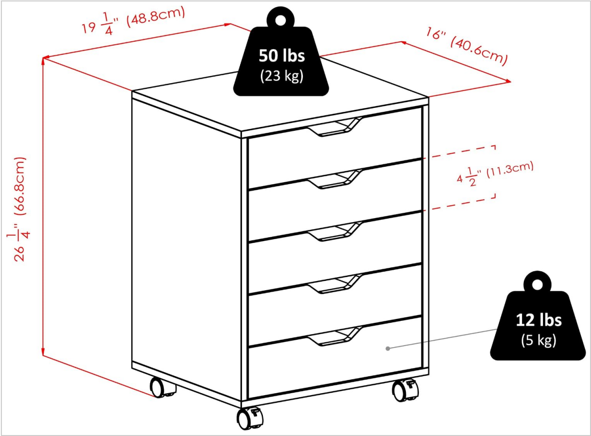
Image 7.1: Dimensional diagram of the cabinet, including overall height, width, depth, and individual drawer dimensions, along with weight capacities.
