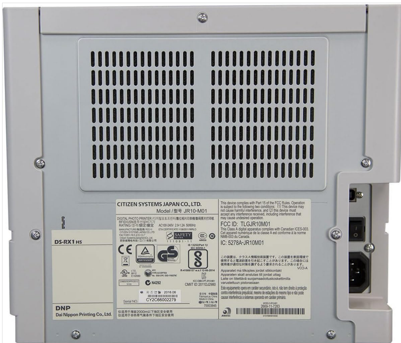
Figure 2: Rear view of the DNP DS-RX1HS Photo Printer. This image highlights the power input and USB connectivity port on the back panel.
