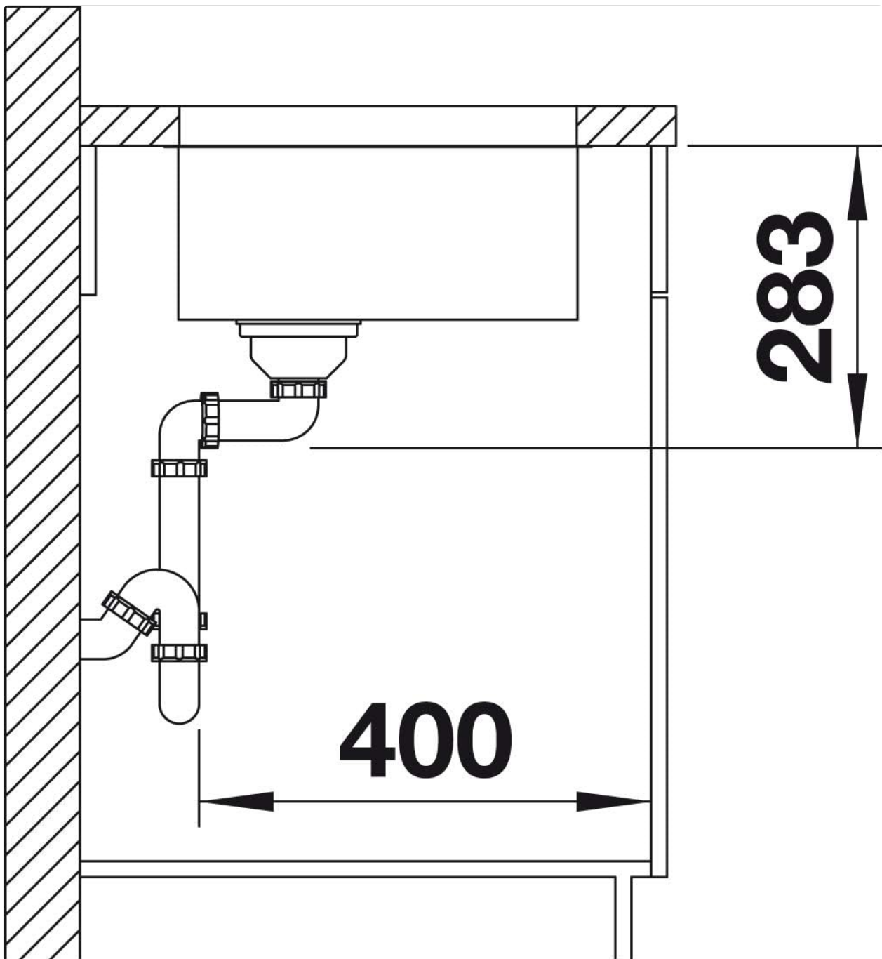
Image 4.3: Detailed side view of the BLANCO Supra 500-U sink with plumbing connections, showing the space-saving pipe and drain assembly.
