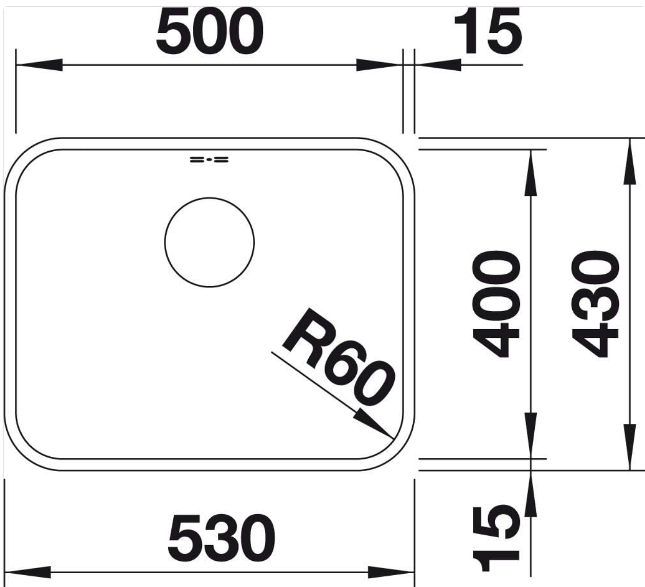
Image 4.4: Top-down dimension diagram of the BLANCO Supra 500-U sink, showing overall length (530 mm) and width (430 mm).
