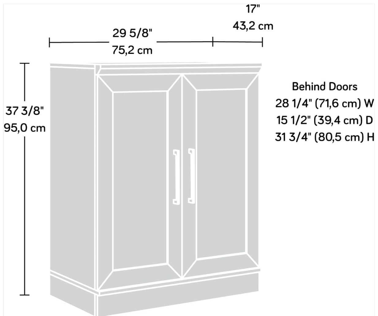
Figure 3: Detailed dimensions of the cabinet.
