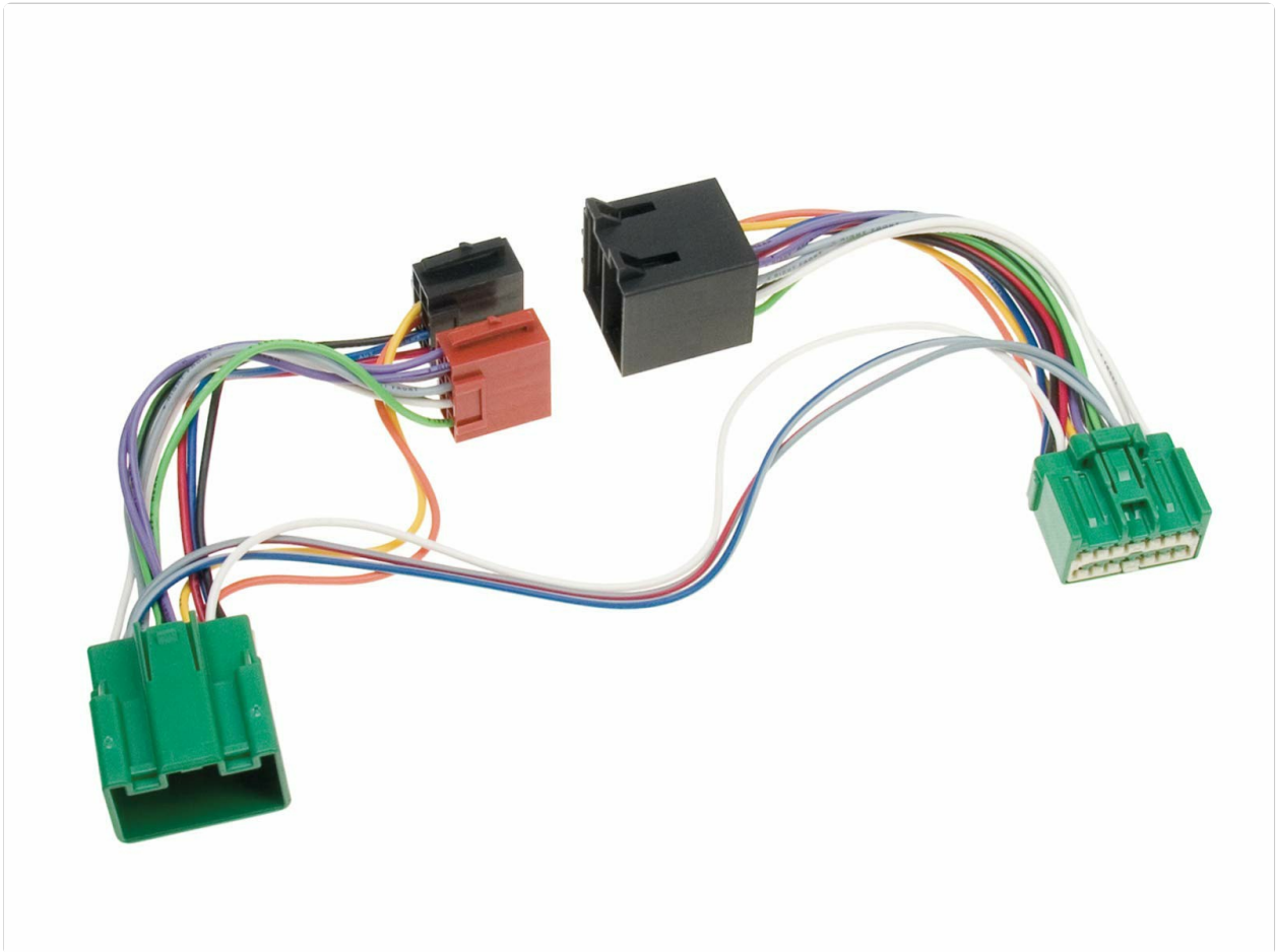
Figure 1: The ACV ISO Wiring Harness Adapter. This image displays the multi-colored wires connecting various black, red, and green plastic connectors, illustrating the adapter's design for connecting different audio components within a vehicle's electrical system.
