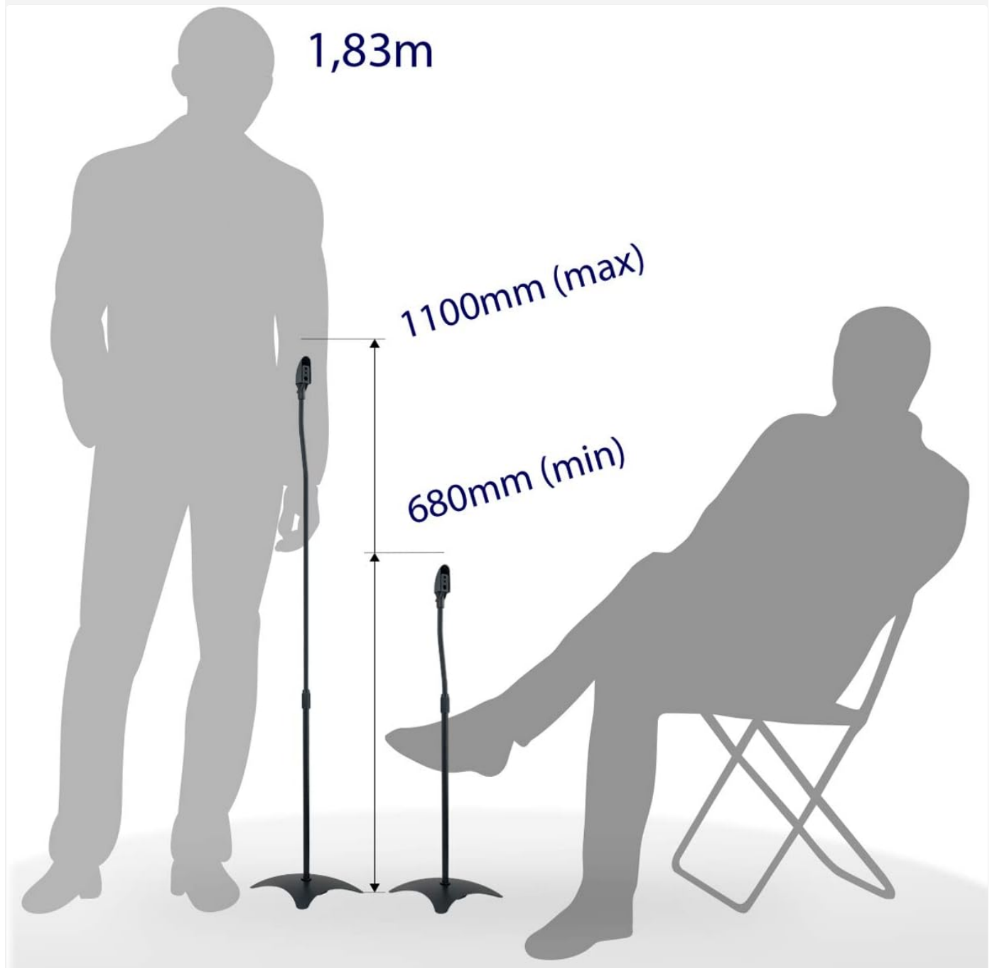
Figure 5.1: Height adjustment range from 680mm (min) to 1100mm (max).
