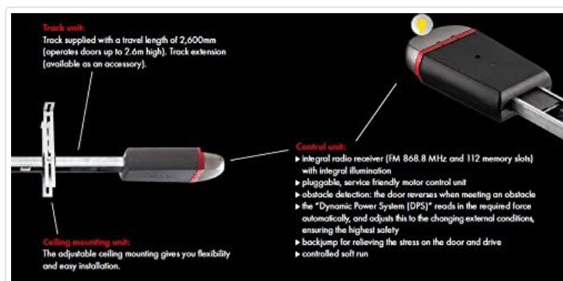
Image 2: Diagram illustrating the track unit, control unit, and ceiling mounting unit with their respective features.
