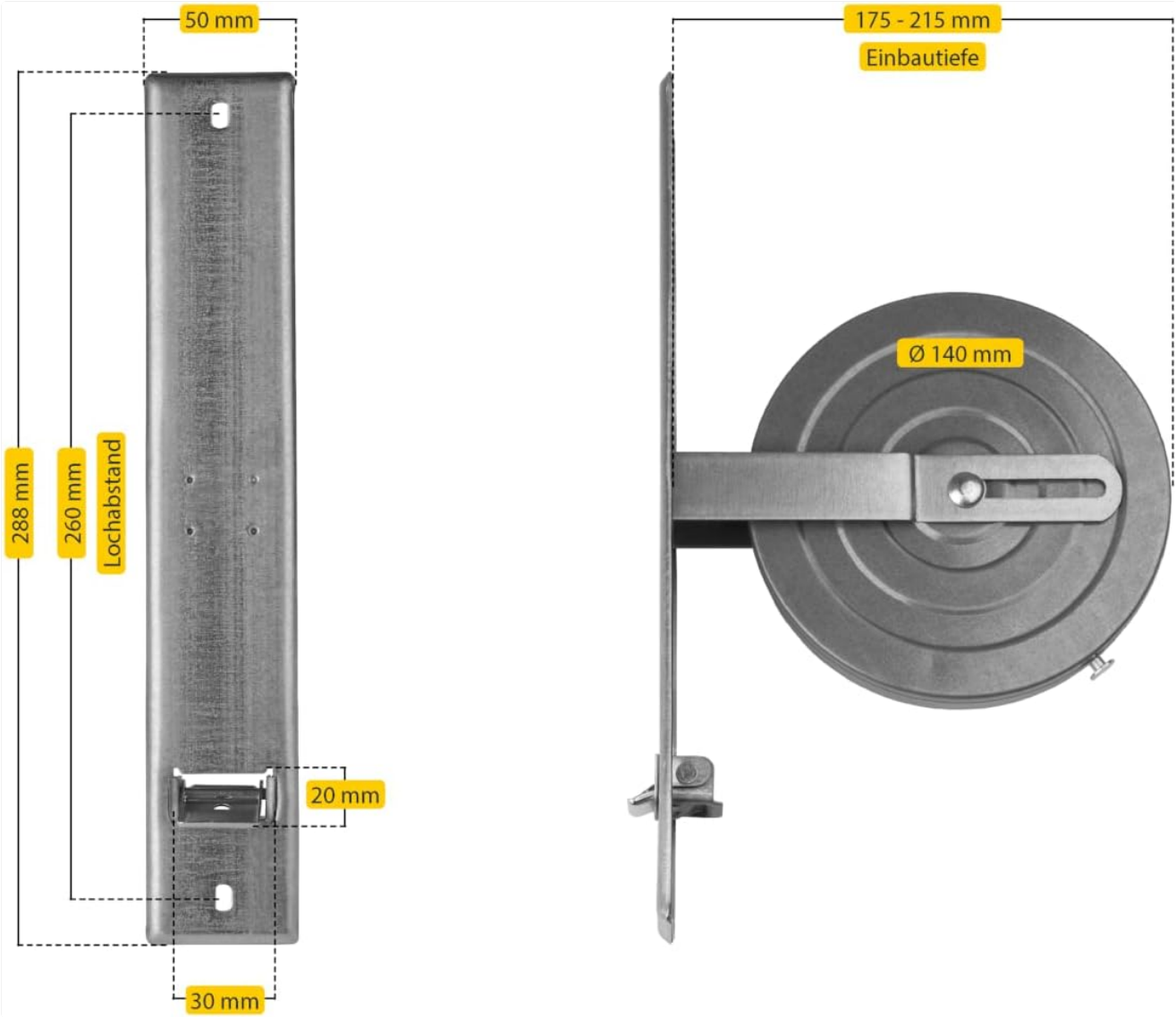
Figure 4: Detailed dimensions of the roller shutter winder for installation planning.
