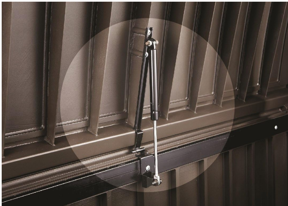
Image 2: A close-up view of the hydraulic piston mechanism, which assists in the smooth opening and soft closing of the deck box lid.
