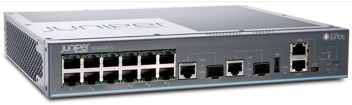
Figure 2: Alternative front view of the Juniper EX2200-C-12T-2G Layer 3 Switch. This perspective offers a clearer view of the port numbering (0-11 for RJ-45 ports) and the labeling of the SFP ports and management interfaces.
