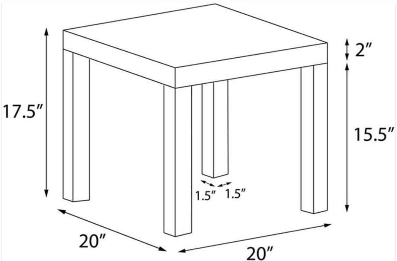
Figure 3.1: Detailed dimensions of the end table for planning placement.
