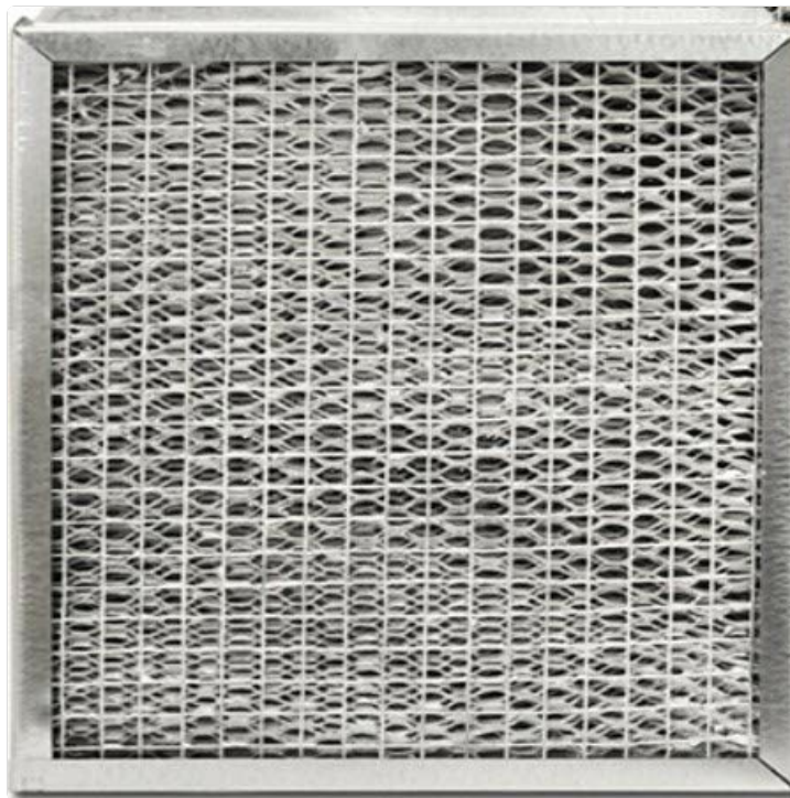
Figure 1.2: Close-up view of the GeneralAire humidifier filter's expanded aluminum base and hydrophilic coating. This material is designed for optimal water absorption and evaporation.
