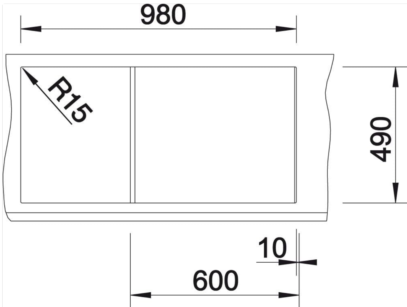
Figure 5: Diagram detailing the countertop cutout dimensions (980mm x 490mm) and corner radius (R15) required for installation.
