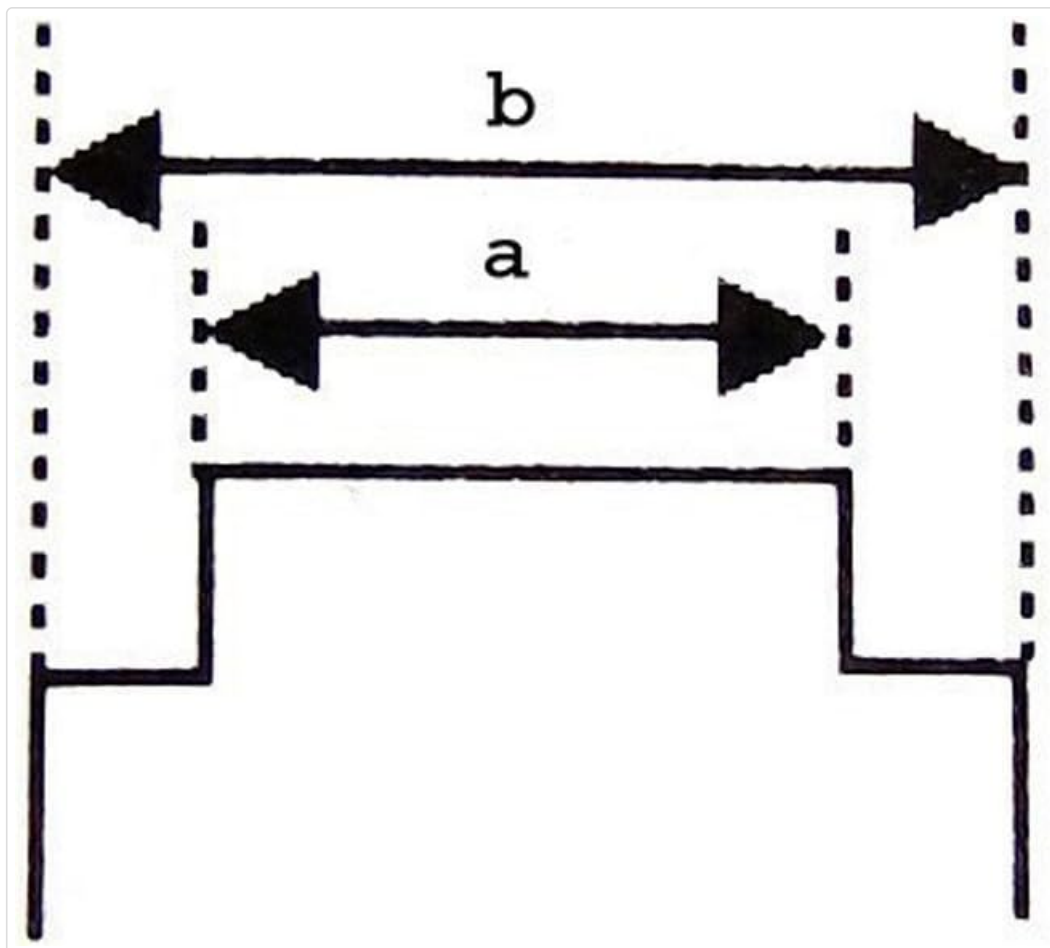
Figure 3: Diagram for measuring lug width (a) and overall strap width (b) for proper fitment.
