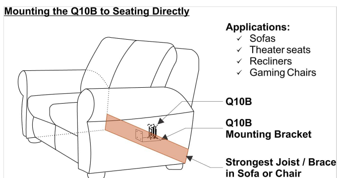
Figure 2: Recommended mounting position on seating structure.
