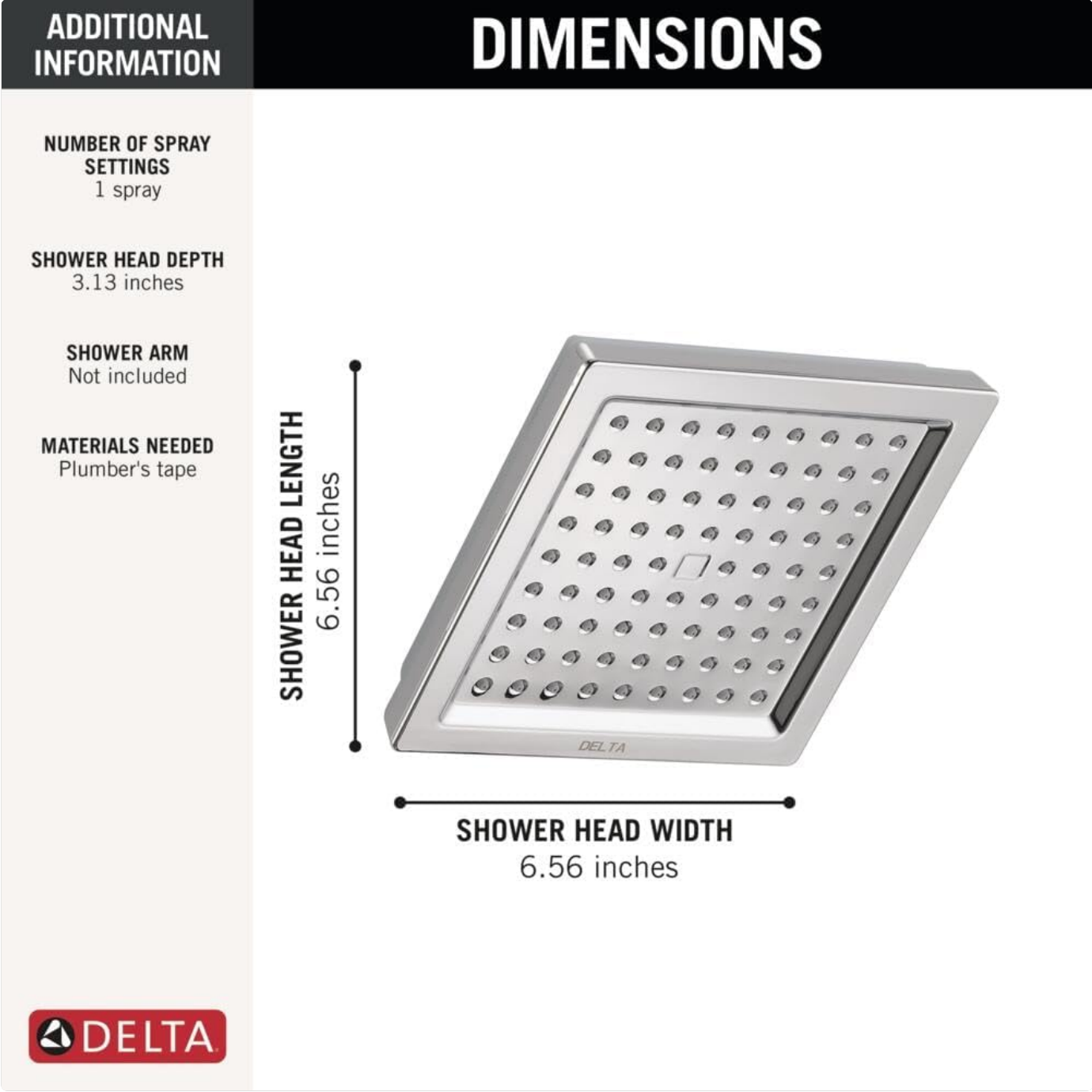
Figure 1: Product Dimensions and Installation Overview. Note that the shower arm is not included.
