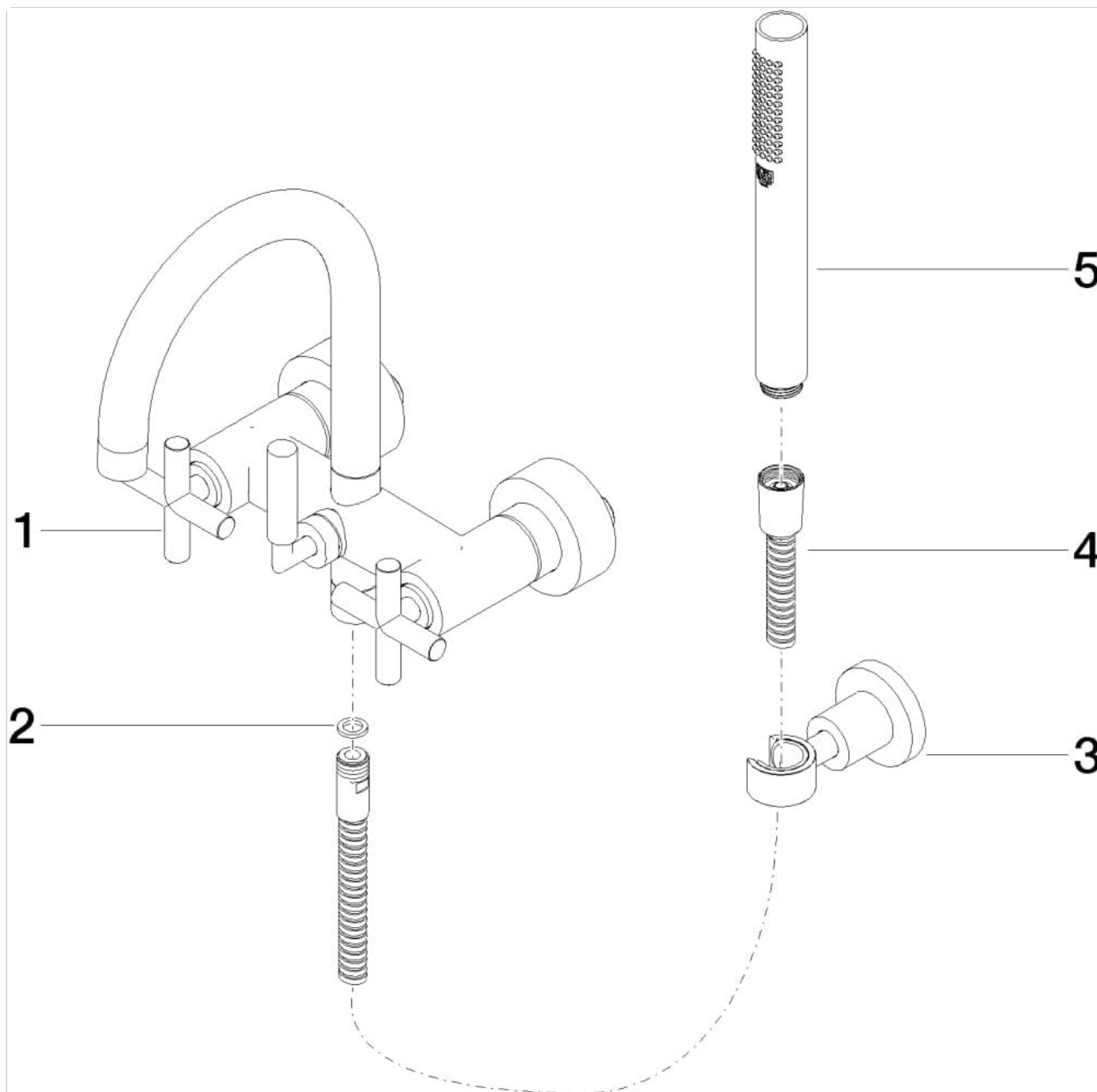
Image 1.1: Dornbracht 25133892-00 Wall-Mounted Bath Mixer with Hand Shower in Chrome finish.
