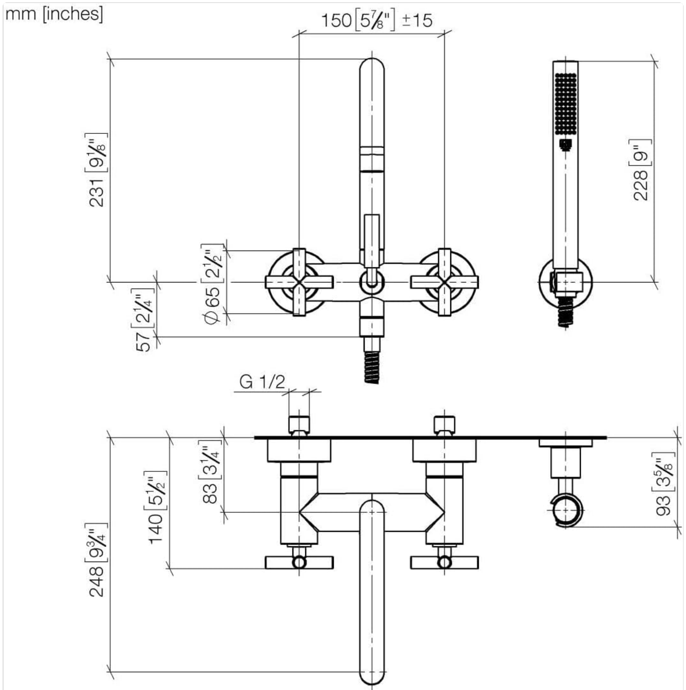
Image 4.1: Dimensional drawing showing key measurements for installation planning. All dimensions are in millimeters and inches.
