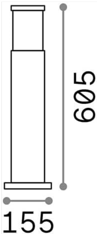
Image: Technical drawing showing the dimensions of the TRONCO PT1 H60 lamp. The height is 605mm and the diameter is 155mm. This diagram is crucial for planning the installation space.
