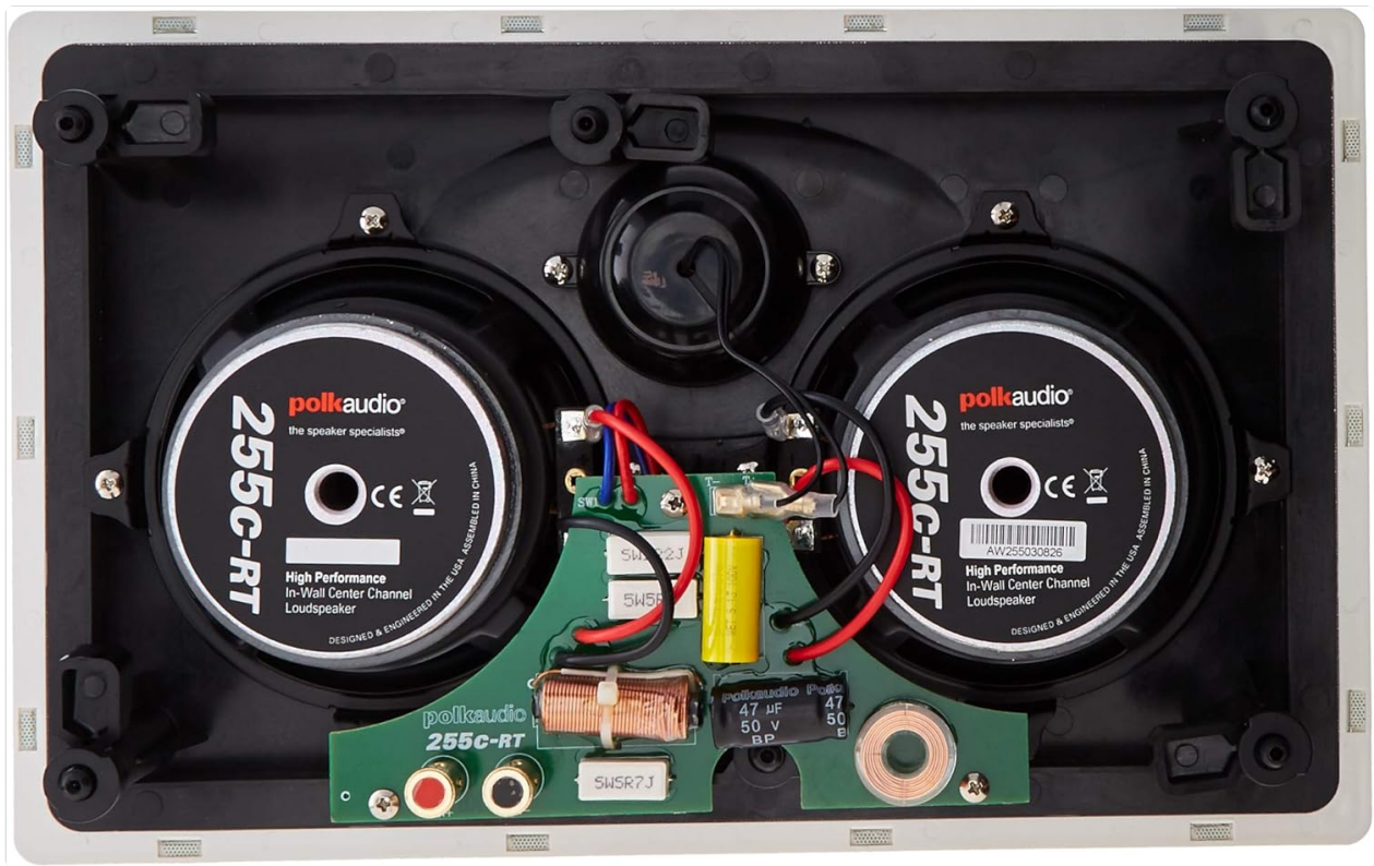
Figure 2: Rear view of the 255c-RT speaker, illustrating the wiring terminals and internal components. This view highlights the Power Port technology and the robust construction.
