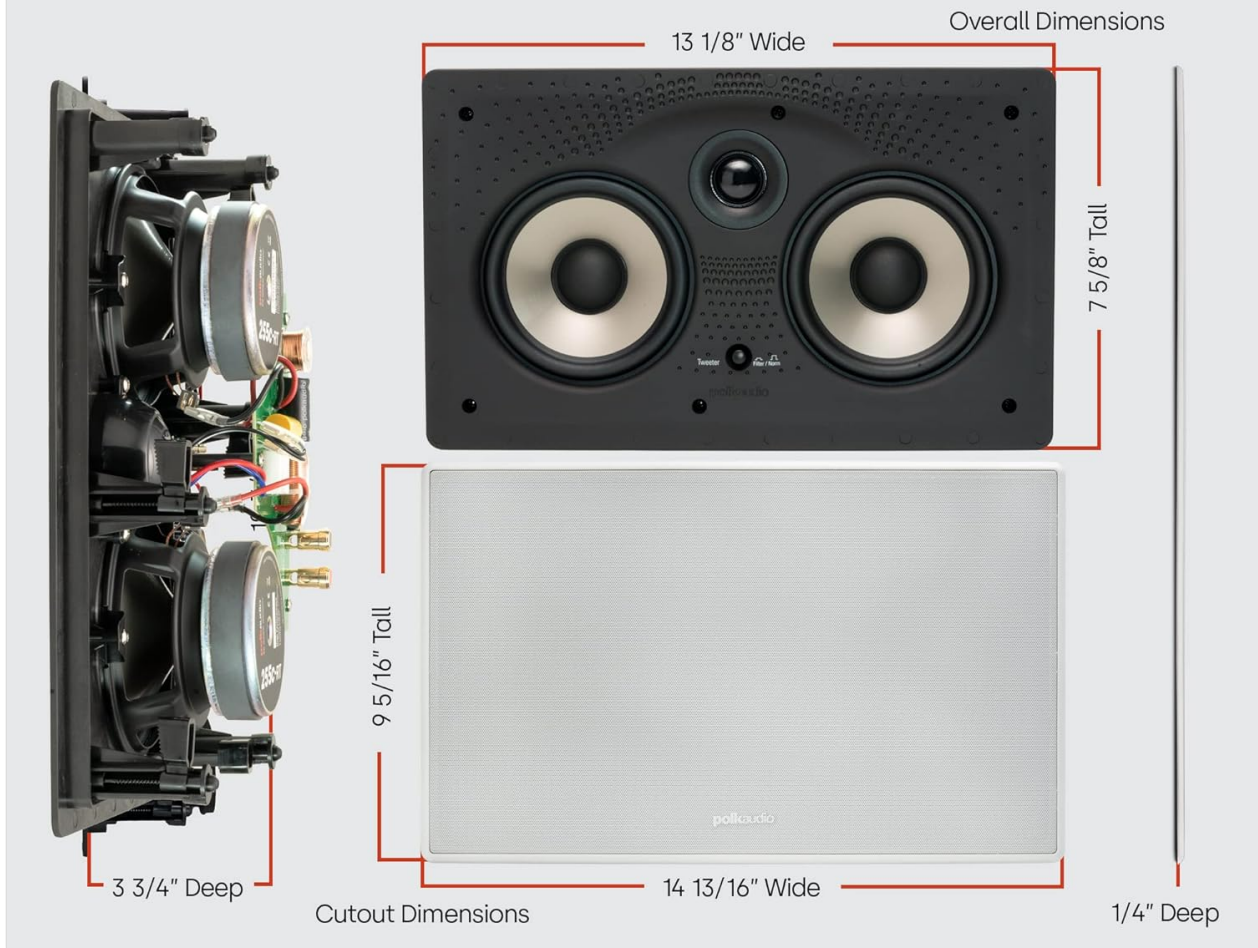
Figure 1: Speaker dimensions and cutout template for installation. The image shows the overall dimensions of the speaker (13 1/8" Wide x 7 5/8" Tall) and the cutout dimensions (9 5/16" Tall x 14 13/16" Wide), along with a depth of 3 3/4".
