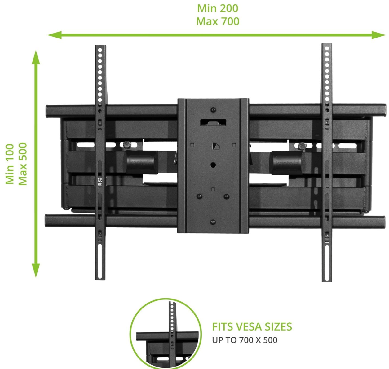
Image: Diagram illustrating the VESA compatibility of the Kanto FMX3C mount, showing minimum and maximum dimensions.
