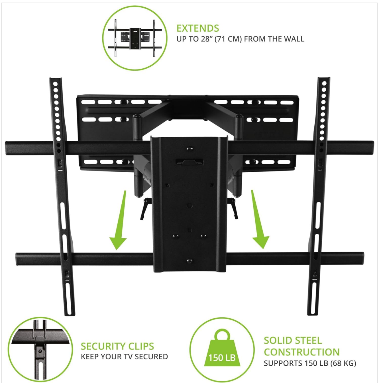
Image: The Kanto FMX3C mount extended, highlighting the security clips that keep the TV secured and its 150 lb weight capacity.
