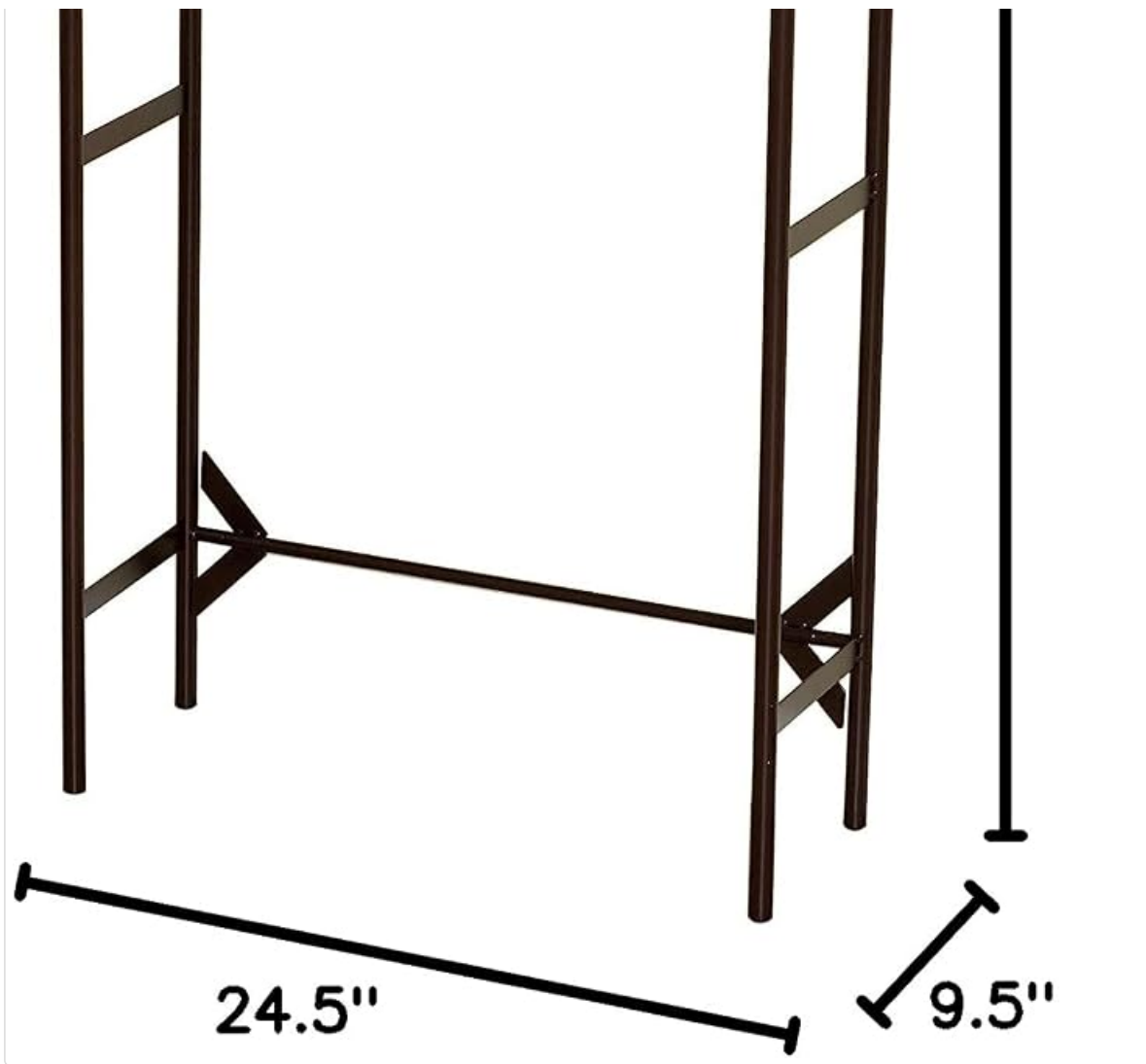
Detailed dimension diagram of the spacesaver, showing 65 inches height, 24.5 inches width, 9.5 inches depth, and 36 inches clearance.
