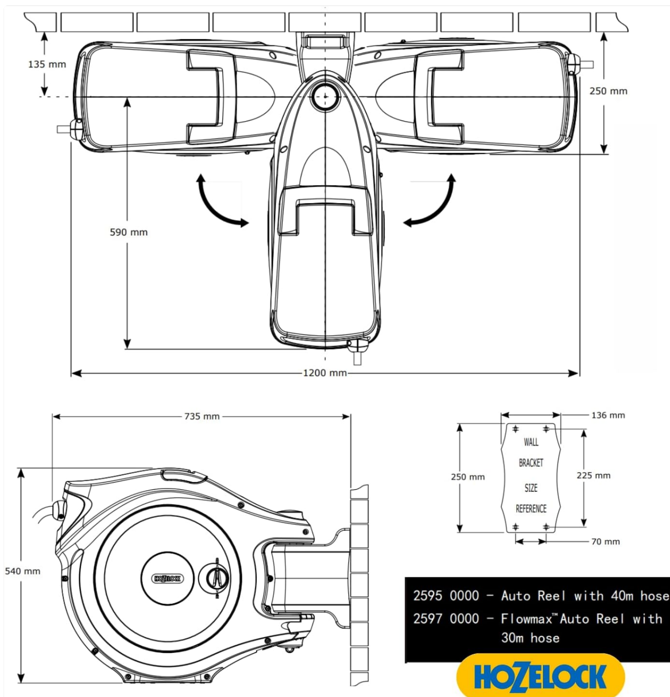
Figure 7: Technical drawing illustrating the dimensions of the Hozelock Auto Reel and its wall bracket.
