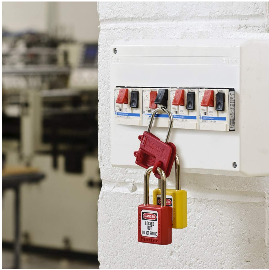
Image 5.1: The Master Lock S430 hasp applied to a circuit breaker panel, secured with two safety padlocks, demonstrating its use in an electrical lockout scenario.
