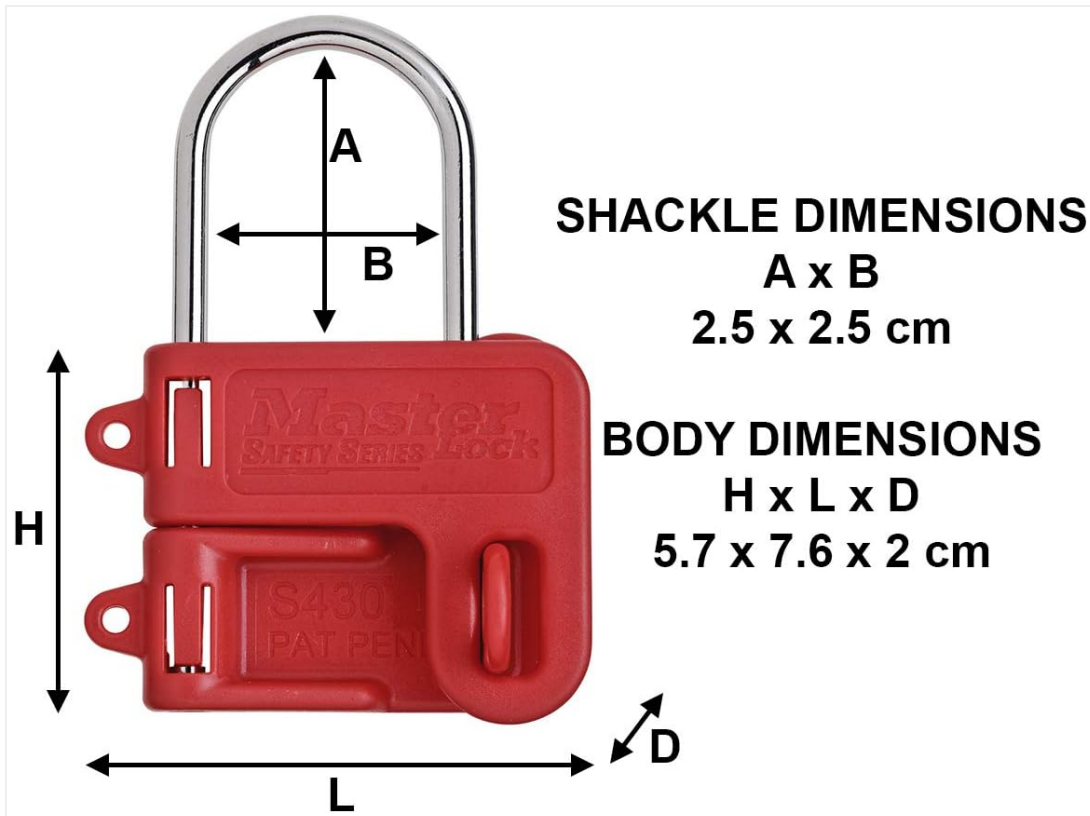
Image 3.1: Detailed diagram showing the shackle and body dimensions of the Master Lock S430 hasp.
