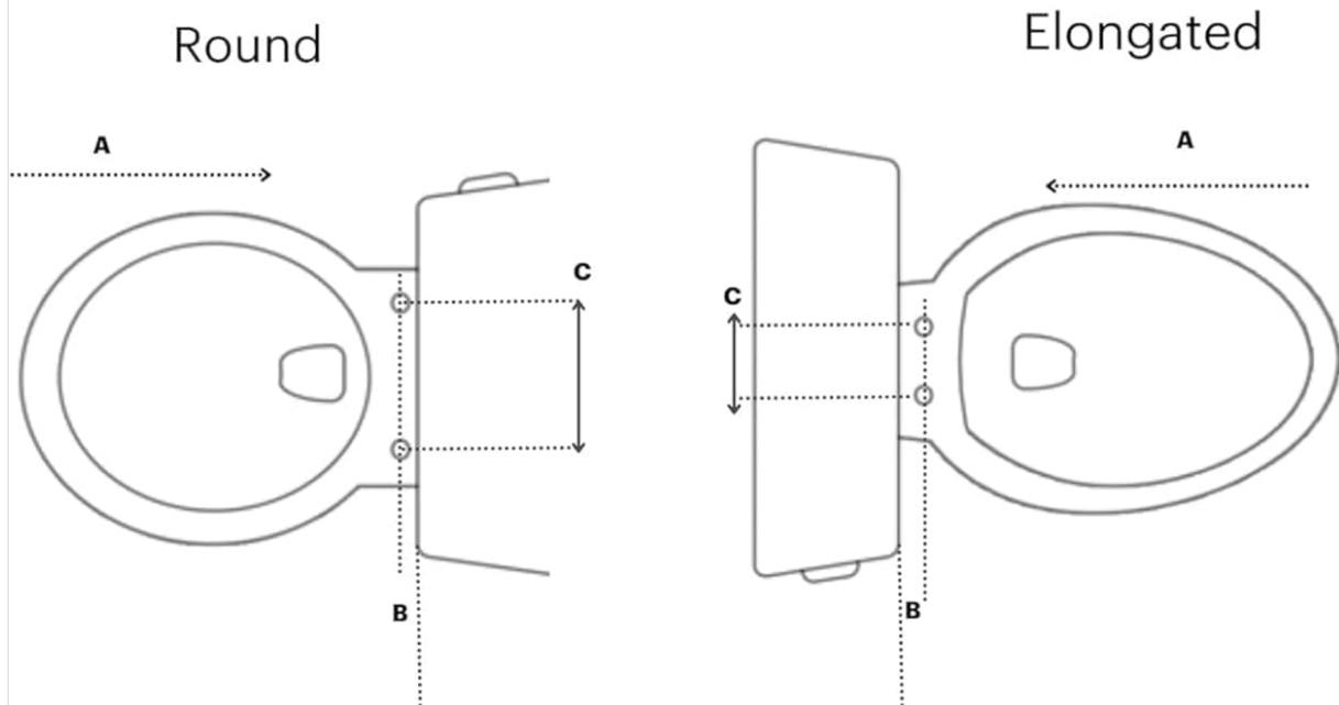
Figure 1: Toilet Measurement Guide for Round and Elongated Seats. This diagram illustrates how to measure your toilet bowl to determine if it is a round or elongated shape and to ensure sufficient space for the bidet seat installation.
