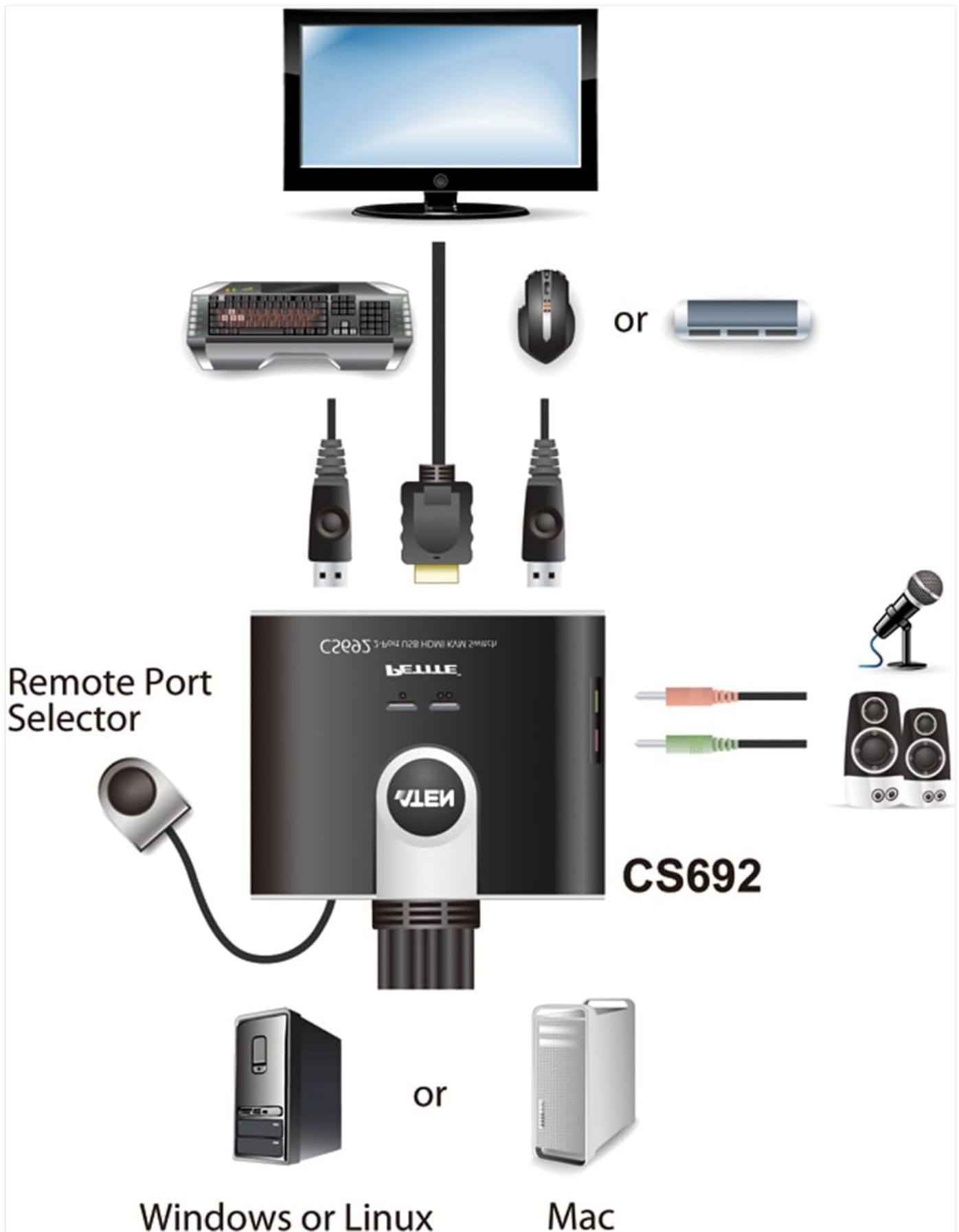
Figure 2: Detailed ATEN CS692 KVM Switch Setup. This diagram provides a more detailed view of the setup, including the KVM unit, the remote port selector, and the connections to the shared monitor, keyboard, mouse, and two distinct computer systems (Windows/Linux and Mac).
