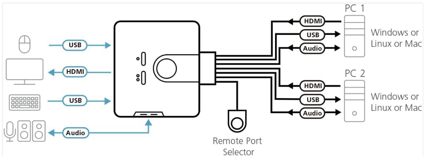
Figure 1: ATEN CS692 KVM Switch Connection Overview. This diagram illustrates how to connect two PCs (Windows, Linux, or Mac) to the KVM switch using HDMI, USB, and audio cables, and how the KVM connects to a single monitor, USB keyboard, USB mouse, and optional speakers/microphone. The remote port selector is also shown.
